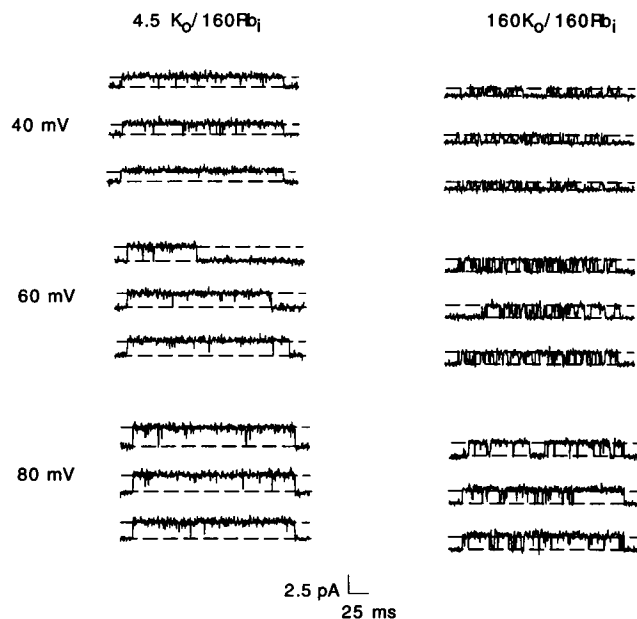
FIGURE 5 Single K^+ currents in outside-out oocyte patches recorded from the M430L mutant at +40, +60, and +80 mV (holding potential of -80 mV) under different ionic conditions. Left: 160 \text{ Rb}_i^+ / 4.5 \text{ K}_o^+ . Right: 160 \text{ Rb}_i^+ / 160 \text{ K}_o^+ .
