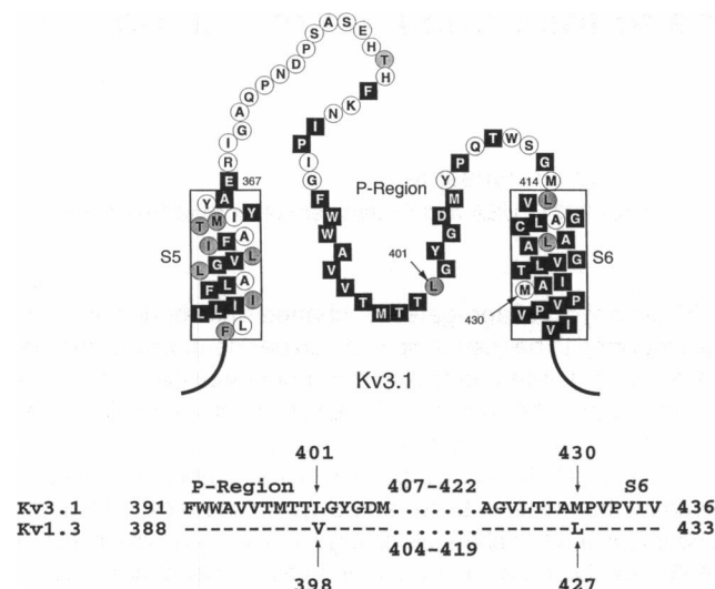
FIGURE 1 (A) The amino acid sequence of Kv3.1 extending from S5 through S6 segments. Black squares: amino acids in Kv3.1 that are identical to those in Kv1.3. Gray circles: residues in Kv3.1 that are replaced by conservative substitutions in Kv1.3. Open circles: residues in Kv3.1 that are dissimilar to those in Kv1.3. (B) Amino acid alignment of the P-region and S6 segment of Kv3.1 and Kv1.3. Dashed lines represent residues in Kv1.3 that are identical to those in Kv3.1. Leucine 401 and methionine 430, the two residues that were mutated, are indicated by arrows.
